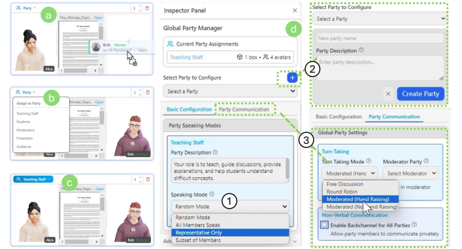
Figure 4: Group dynamics authoring. In the Scene Panel, users can (a) drag participants and/or contents; (b-c) configure the formation of parties via the interactive boxes; (d) tune the speech and turn-taking behaviors of the parties via the Inspector Panel.
