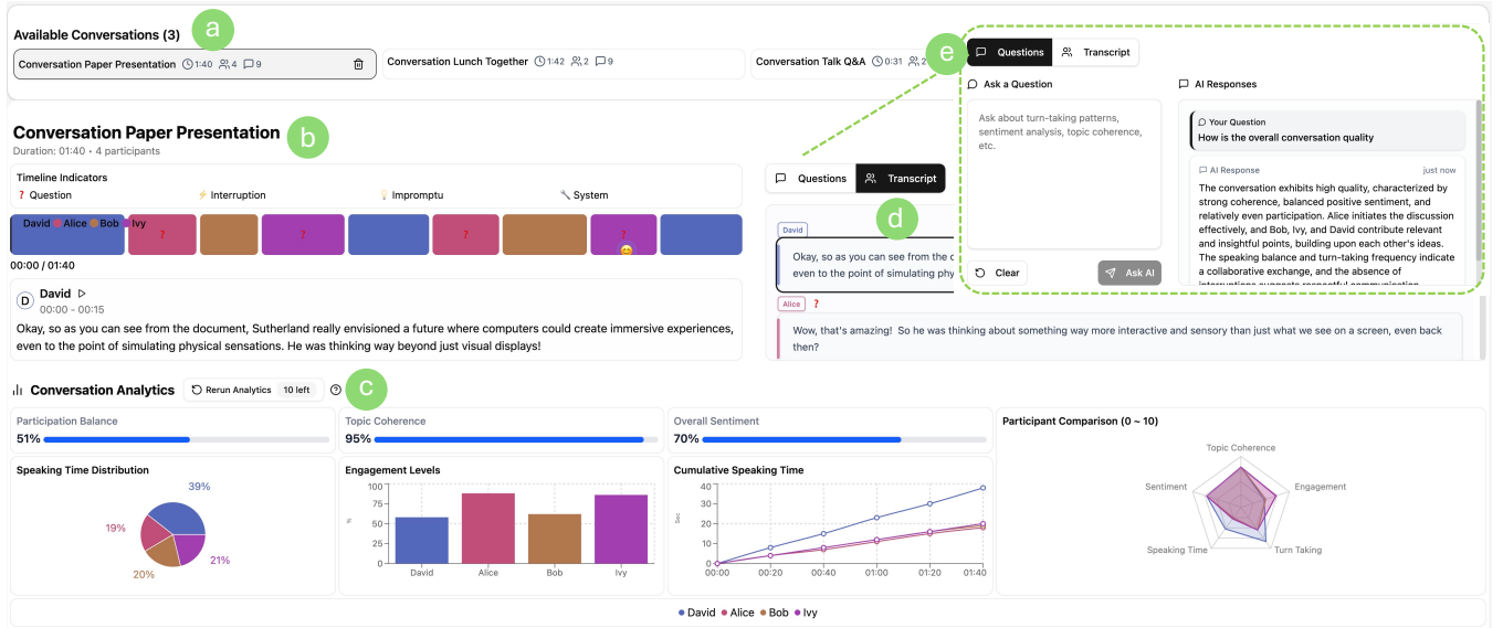
Figure 8: The Verification Dashboard supports structured review and reflection through four integrated panels: (a) conversation selector, (b) interactive timeline of speaker turns and key events, (c) analytics panel with visual metrics, (d) synced transcript viewer, and (e) natural language Q&A interface for querying conversation dynamics.
