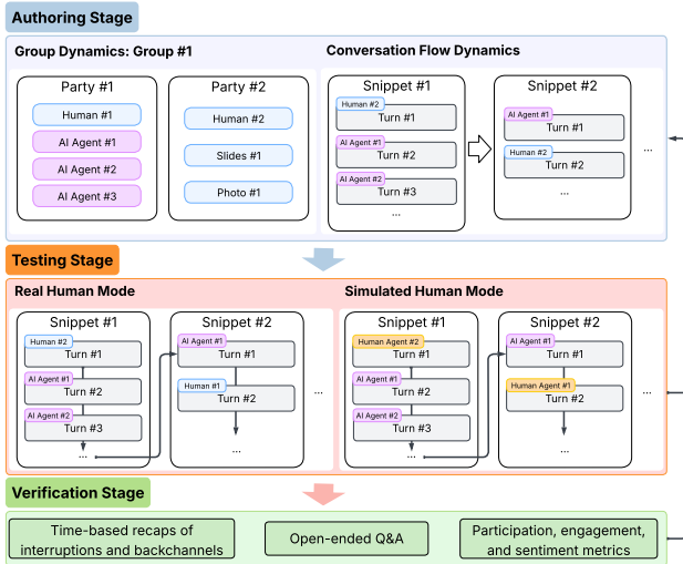
Figure 2: DialogLab workflow: (1) A conversation creator begins with the authoring stage , defining the group dynamics and conversation flow dynamics . (2) The testing stage allows testing the conversation either by involving a human user in the conversation ( real human mode ) or simulating a human user using an agent ( simulated human mode ). (3) In the verification stage , DialogLab generates structured analysis through recap, queries, and analytics. The creator may iterate on the authoring process based on insights from both testing and verification stages until satisfied.
