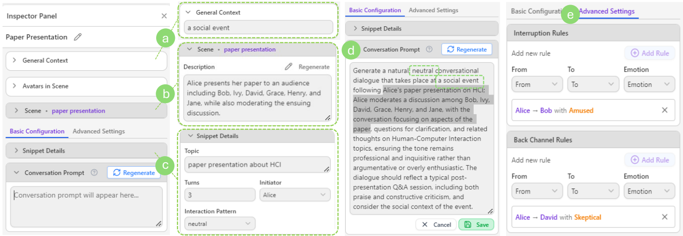
Figure 5: The configuration of the snippets in the Inspector Panel. It includes: (a) a general context field that defines the situational backdrop (e.g., "a social event"); (b) the automatically updated scene description; (c) snippet details, including topic, number of turns, initiator, and interaction pattern; (d) an editable conversation prompt, auto-generated by combining the general context, scene description, and snippet details; (e) Advanced Settings, where users can configure interruption and backchannel rules between characters, along with associated emotional tones.
