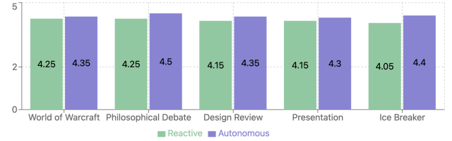
Figure 14: Average ratings comparison between Reactive and Autonomous modes across different conversation topics.
